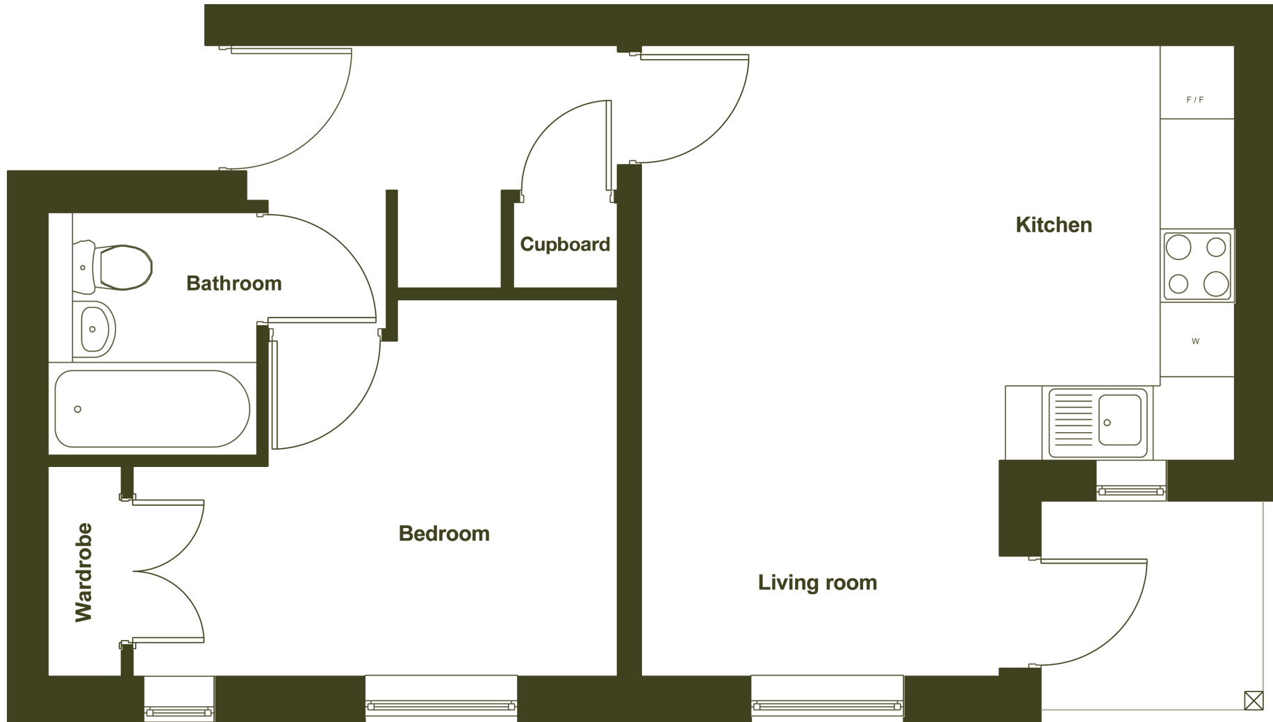
BLOCK G GROUND FLOOR PLAN
