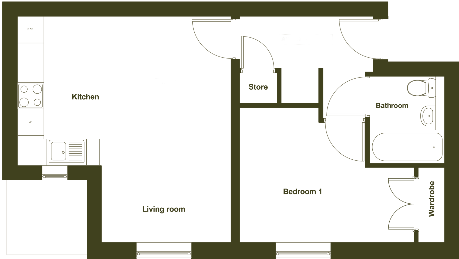
BLOCK H THIRD FLOOR PLAN
